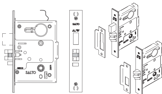
Model LA1M1770 standard ANSI
